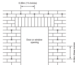
2 Door and window frame drilling pattern
