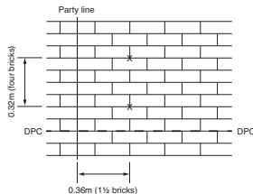
4 Drilling pattern at a party wall
